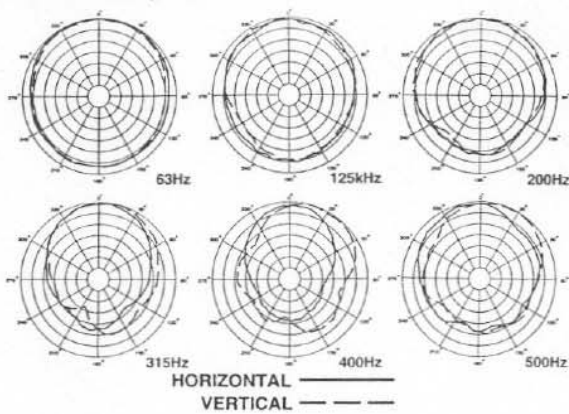
FIGURE 4 — Polar Response
